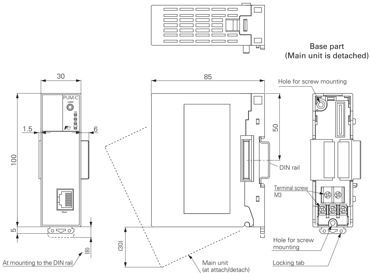
Dimensions for screw mounting
