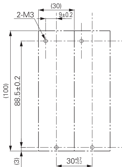
Dimensions for screw mounting
